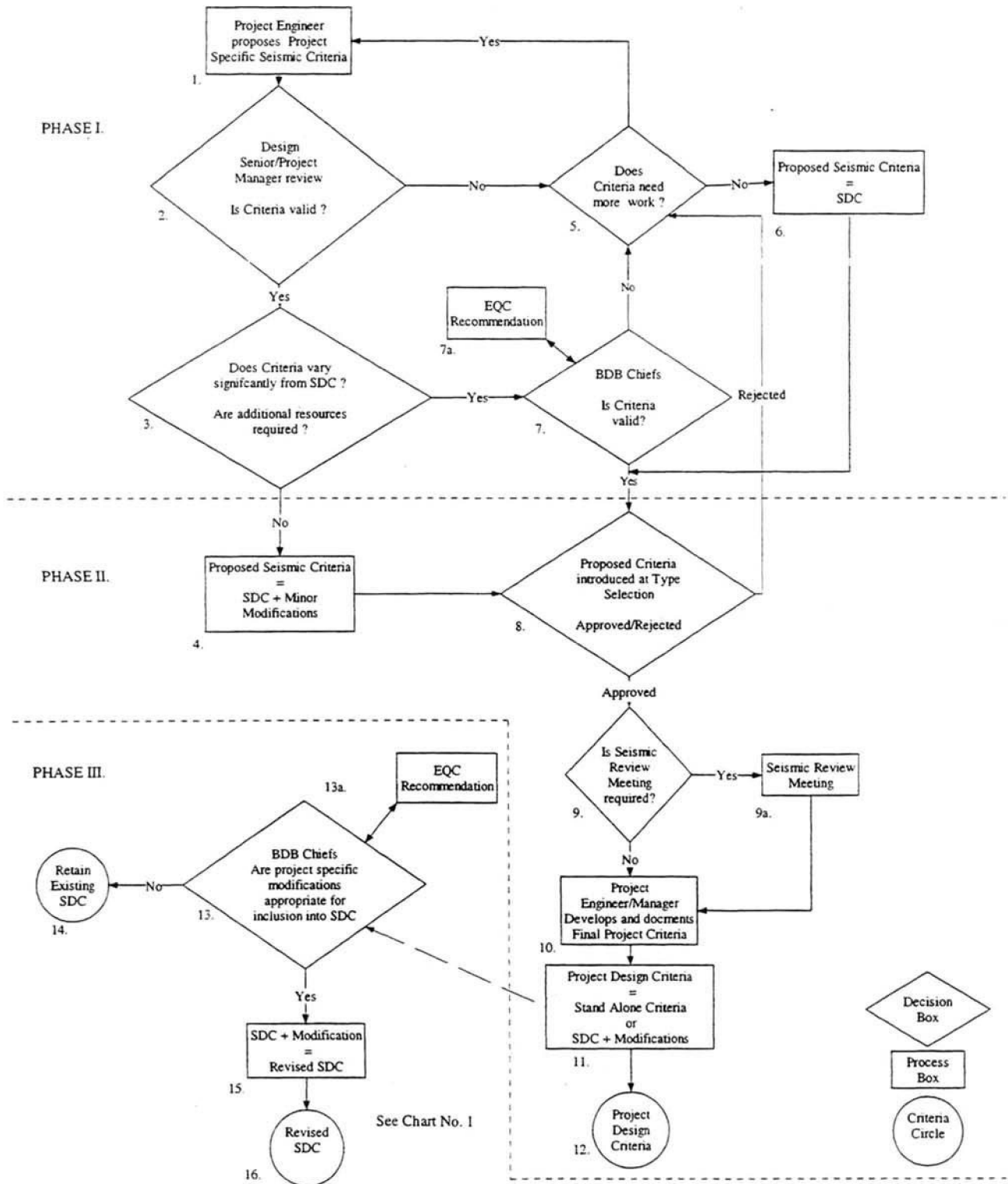
Chart No. 2 - Caltrans Bridge Seismic Design Criteria Development/Retention (Associated with a PS&E Package)
