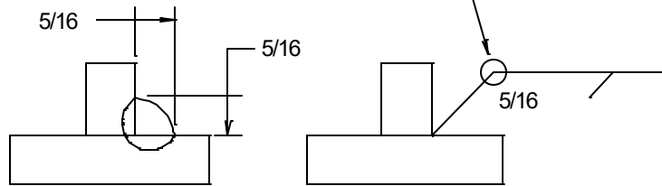
SIZE OF SINGLE FILLET WELD
