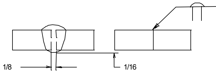
SQUARE-GROOVE WELD
