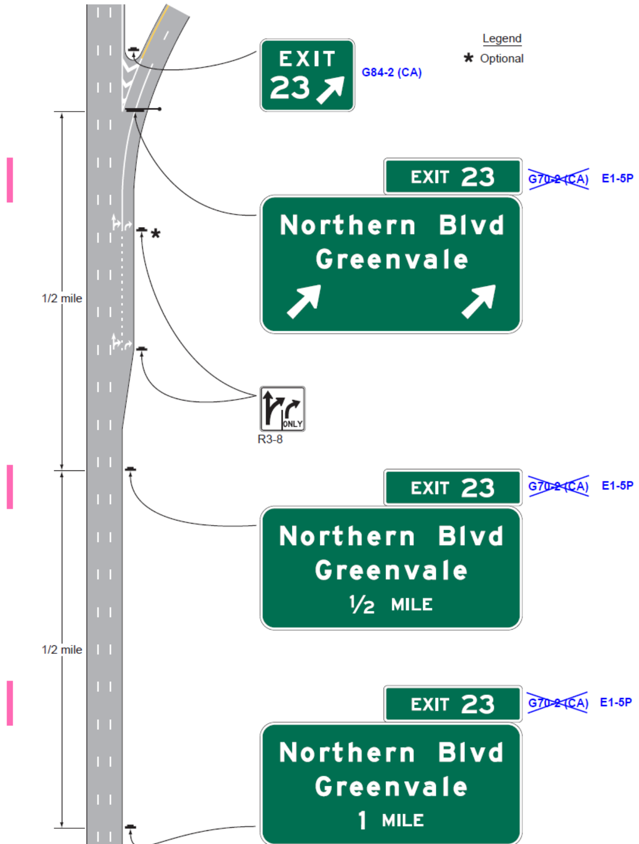
Figure 2E-12. Example of Signing for a Two-Lane Intermediate or Minor Interchange Exit with Option and Auxiliary Lanes
