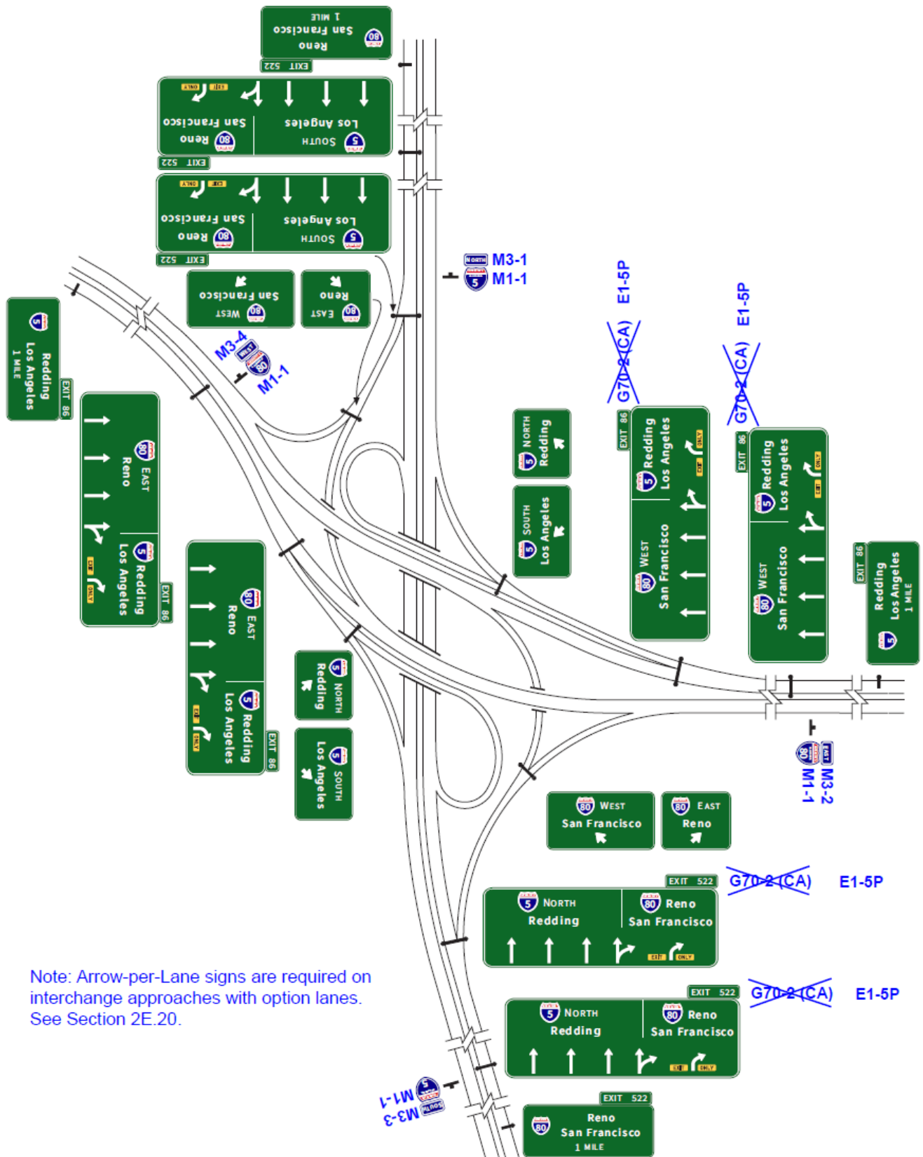
Figure 2E-34 (CA). Examples of Guide Signs for a Freeway-to-Freeway Interchange
