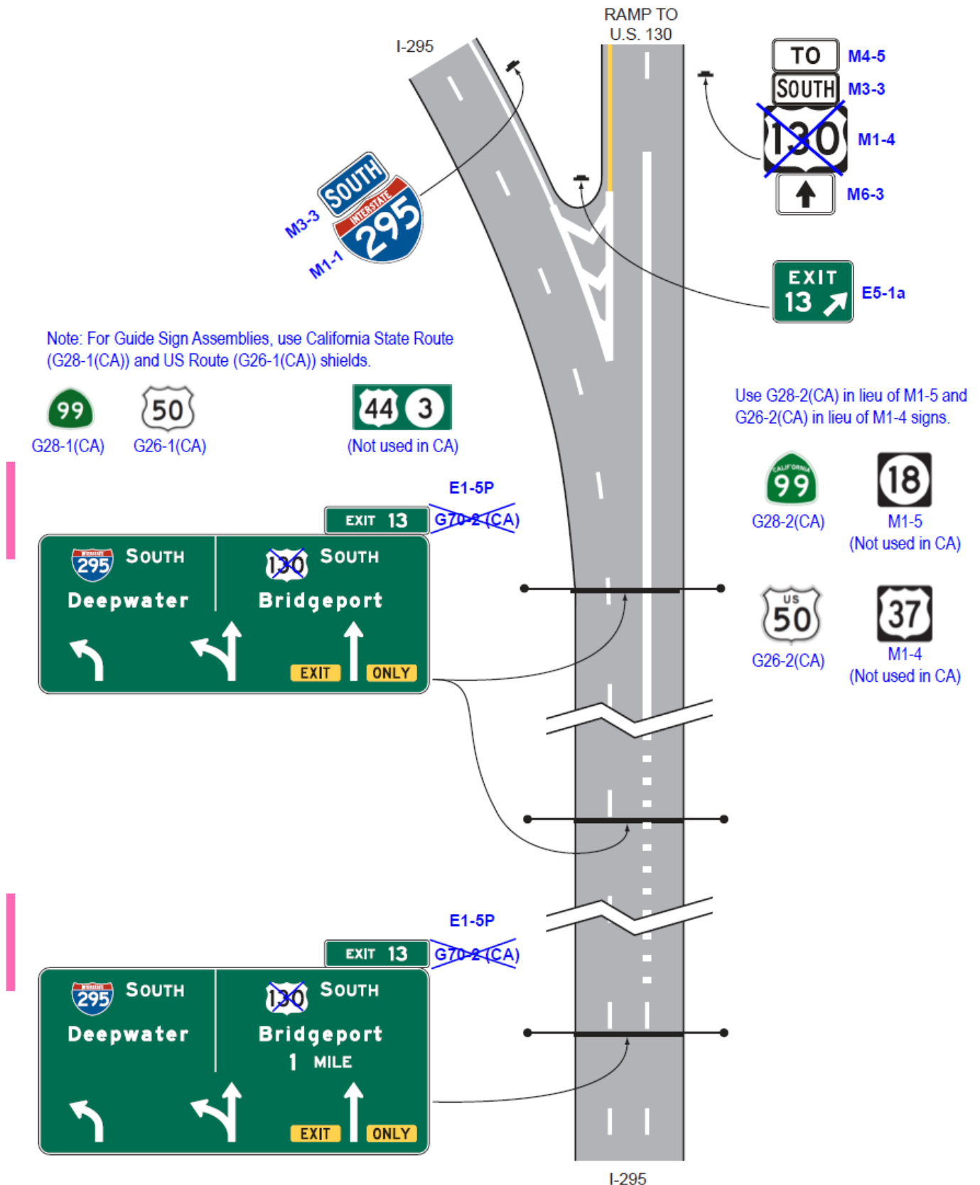
Figure 2E-5. Overhead Arrow-per-Lane Guide Signs for a Two-Lane Exit to the Right with an Option Lane (Through Lanes Curve to the Left)
