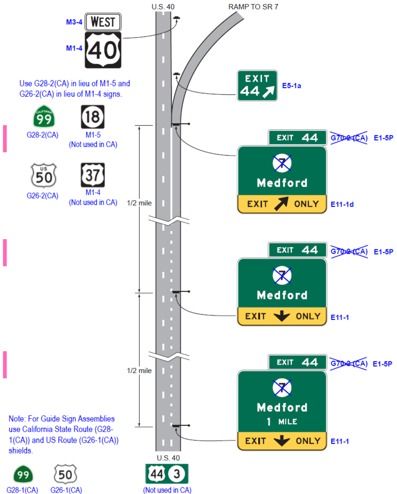
Figure 2E-16. Guide Signs for a Single-Lane Exit to the Right with a Dropped Lane
