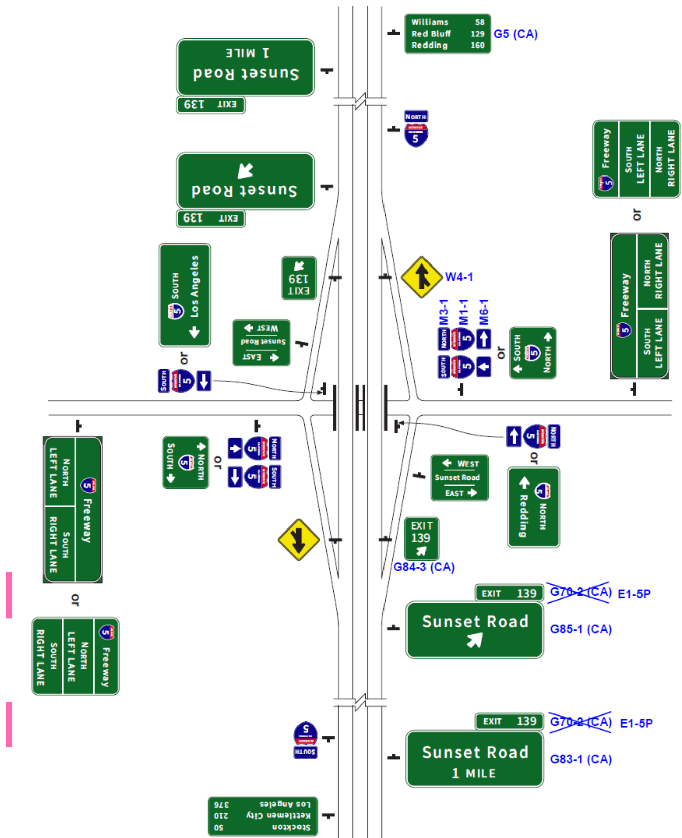
Figure 2E-38 (CA). Examples of Guide Signs for a Diamond Interchange
