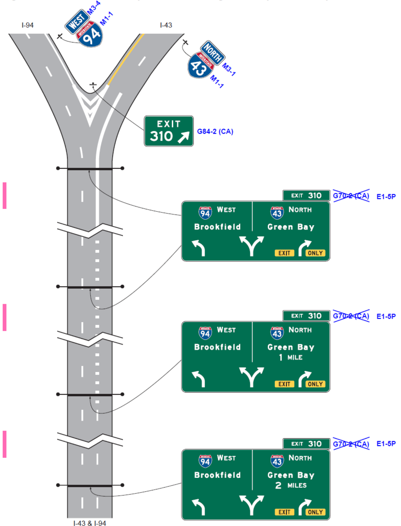
Figure 2E-6. Overhead Arrow-per-Lane Guide Signs for a Split with an Option Lane
